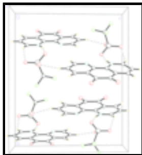
Fig. 2. The molecular packing of (I) viewed approximately along the b axis. Dotted lines indicate the hydrogen bonding interactions.
